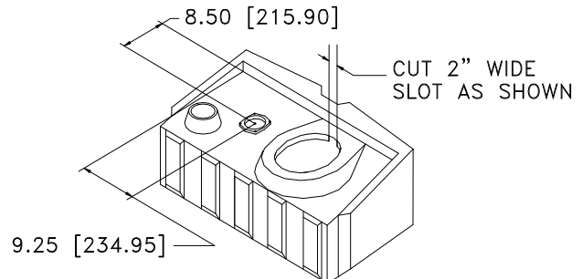
#10553 TUFWAY TANK
