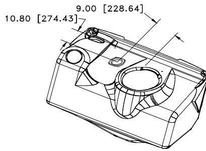
#18934 TAURUS TANK
