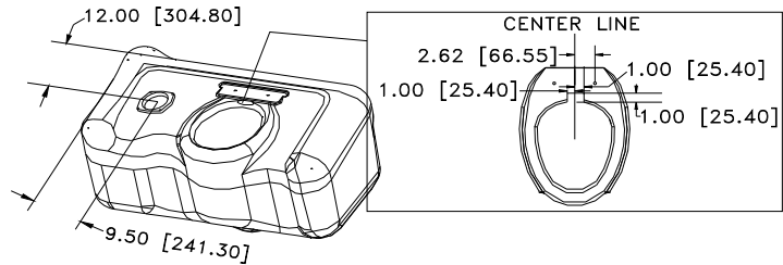
#40017 GLOBAL TANK
