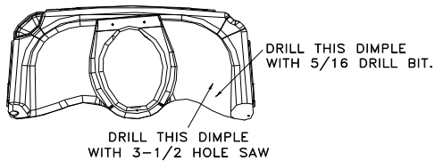
#16690 MX3 TANK
